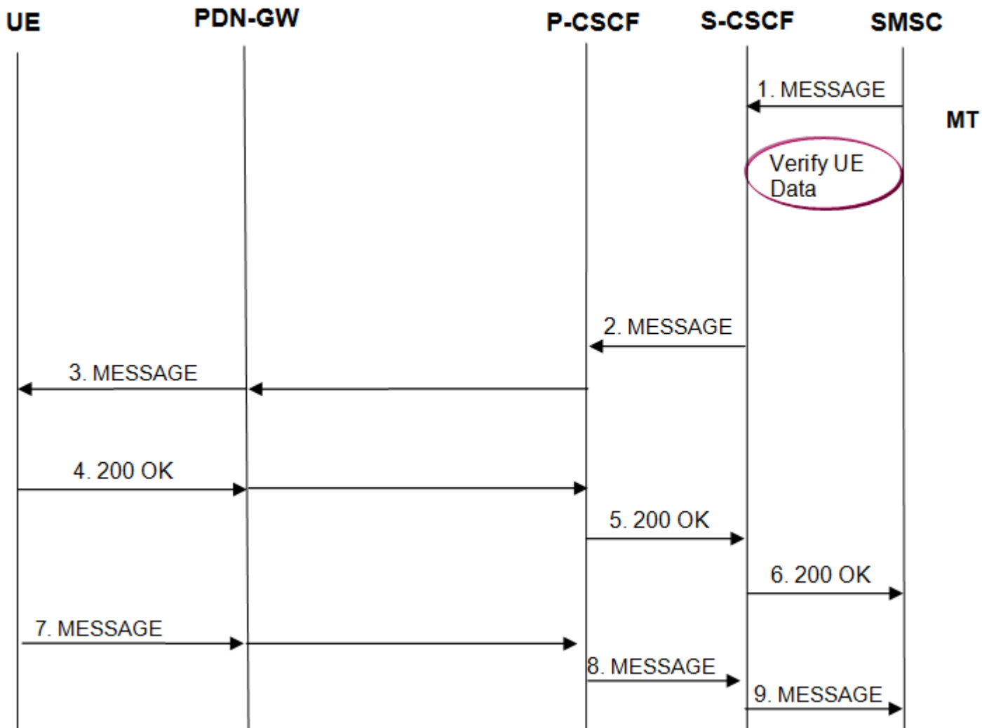
Figure 4: Mobile Terminated 3GPP SMS Call Flow
