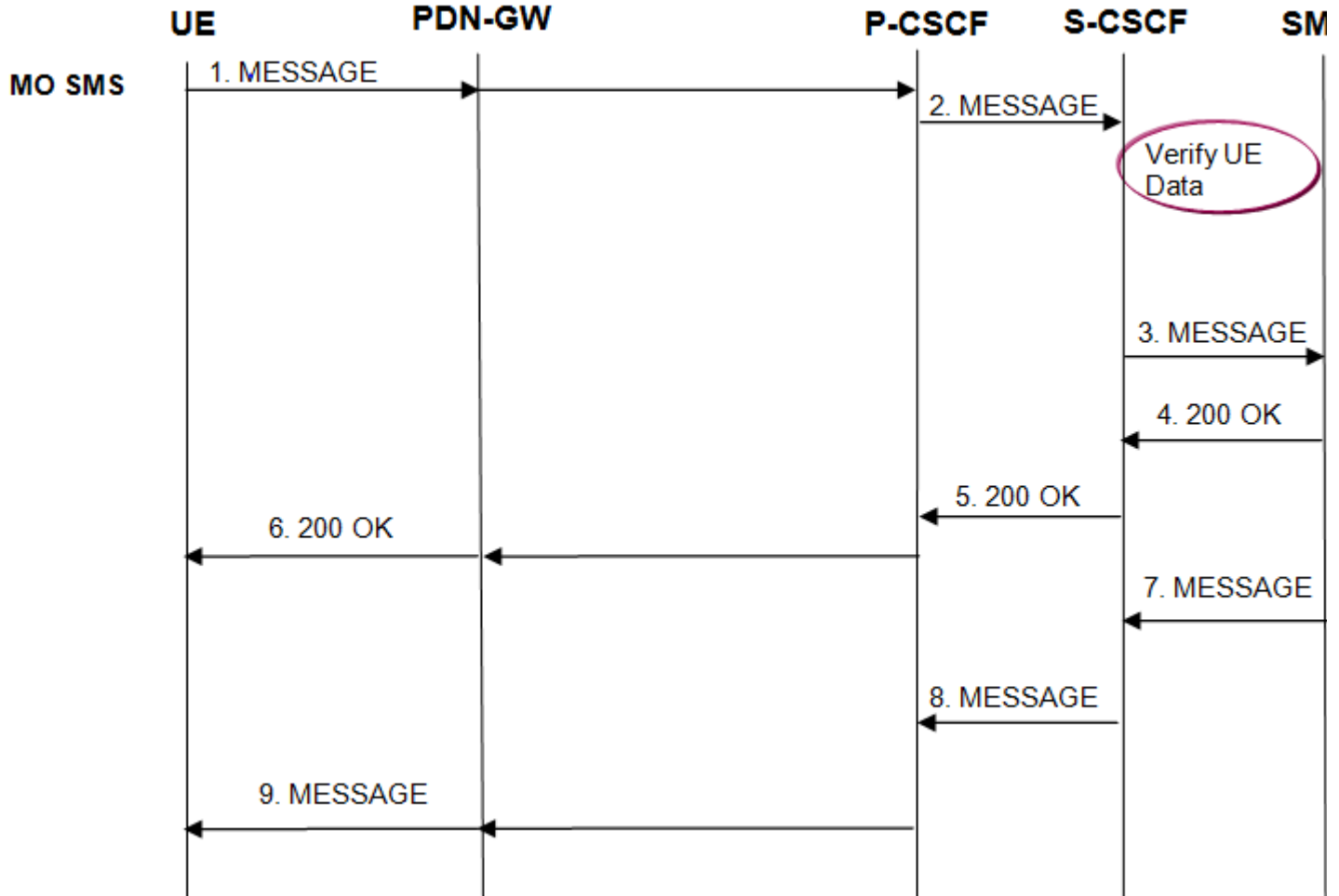
Figure 3: Mobile Originated 3GPP SMS Call Flow
